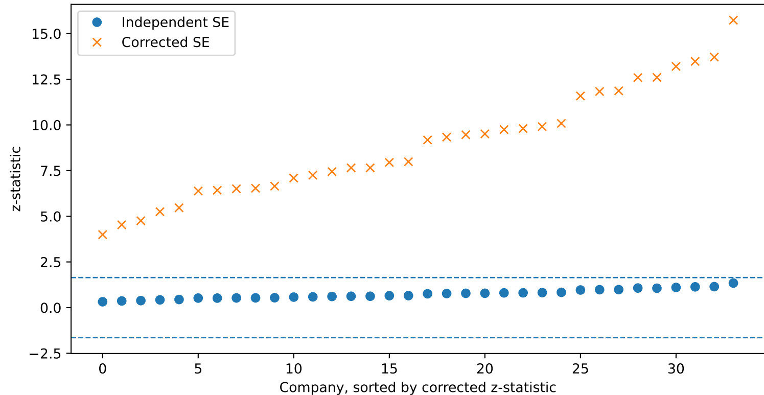
Correcting the covariance changes the proxy-discrimination test
